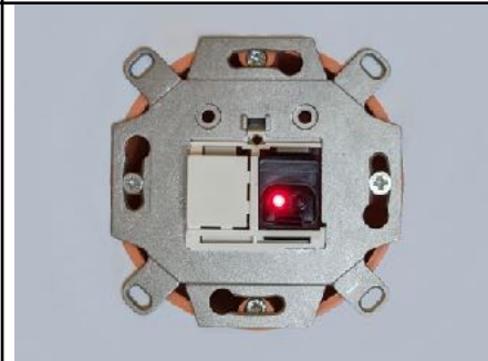
FIX THE KEYSTONE MODULE WITH THE MOUNTING FRAME
